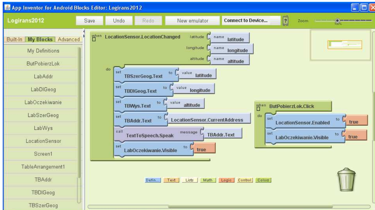
Rys.4. Widok App Inventor Blocks Editor
