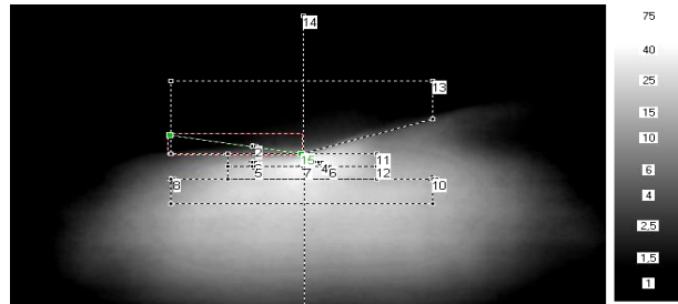
Fig.8. The view of a light spot of low beam light reflector RE03210 (R2) together with indicated places of luminance measurement
