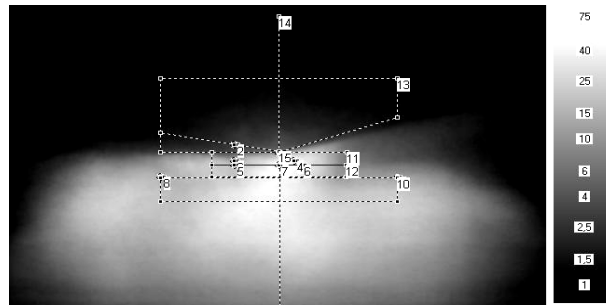
Fig.14. The view of a light spot of main light reflector RE03210 (H4) together with indicated places of luminance measurement
