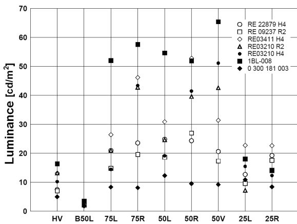
Fig. 15. Luminance measurement results in measurement points of low beam light beams
