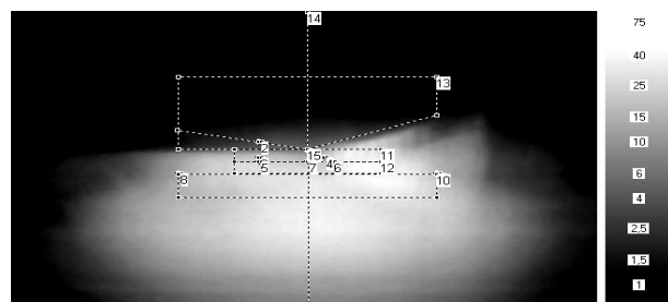
Fig.10. The view of a light spot of low beam light reflector RE22879 (H4) together with indicated places of luminance measurement
