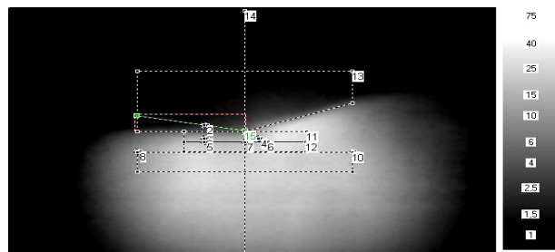
Fig.6. The view of a light spot of low beam light reflector RE09237 (R2) together with indicated places of luminance measurement
