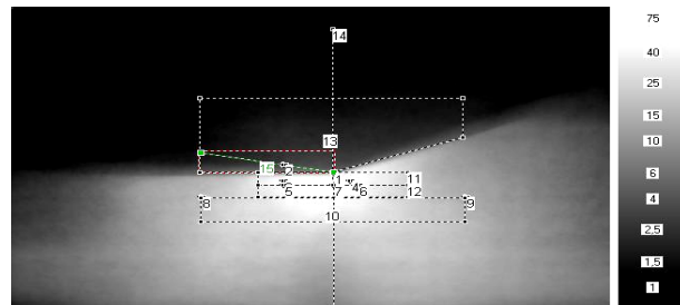
Fig.2. The view of a light spot of low beam light projector 1BL-008 (H7) together with indicated places of luminance measurement
