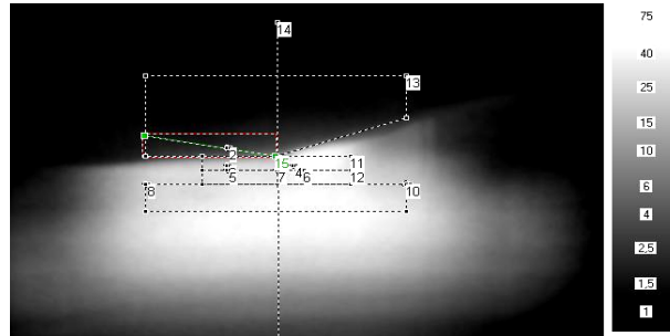
Fig.12. The view of a light spot of low beam light reflector RE03411 (H4) together with indicated places of luminance measurement
