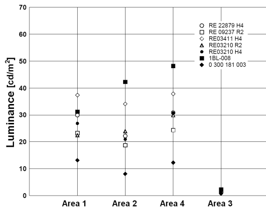
Fig. 16. Luminance measurement results in measurement areas of low beam light beams
