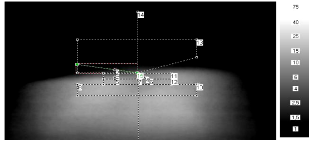
Fig.4. The view of a light spot of low beam light reflector 0 - 300-181-003 (BA20D) together with indicated places of luminance measurement
