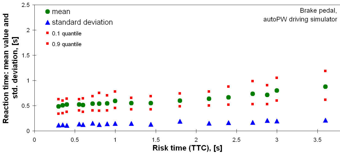
Fig. 8. Reaction time on the brake pedal for scenario I, in driving simulator
