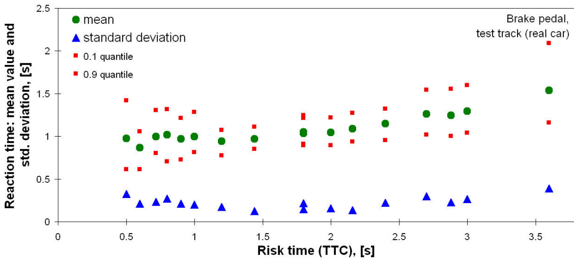
Fig. 9. Reaction time on the brake pedal for scenario I, tests on the track
